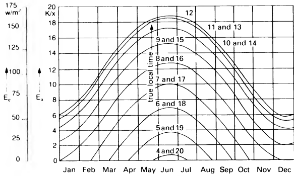
30 Horizontal illuminance E_a for a cloudy sky at latitude 51^\circ\text{N} , as a function of time of year and time of day; E_e = horizontal irradiance
